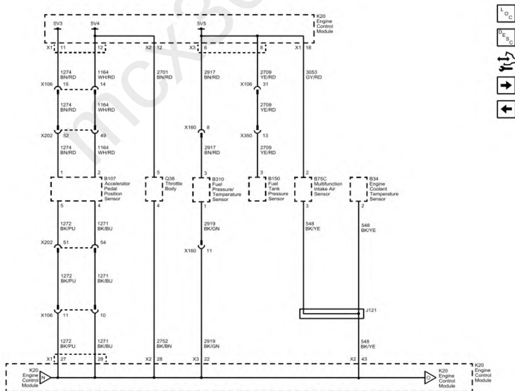
Fig. 3: 5V3, 5V4, 5V5, and Low Reference Bus (2 of 3) Courtesy of GENERAL MOTORS COMPANY
