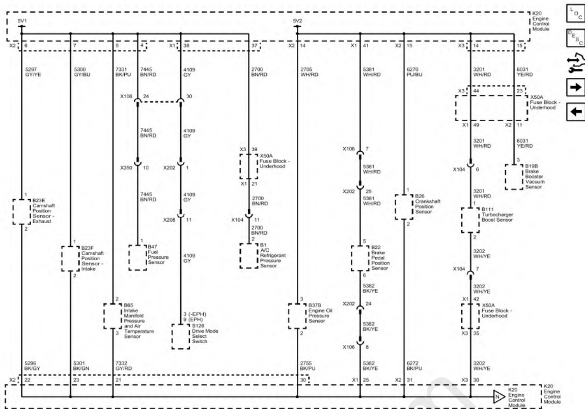
Fig. 2: 5V1, 5V2, and Low Reference Bus (1 of 3) Courtesy of GENERAL MOTORS COMPANY
