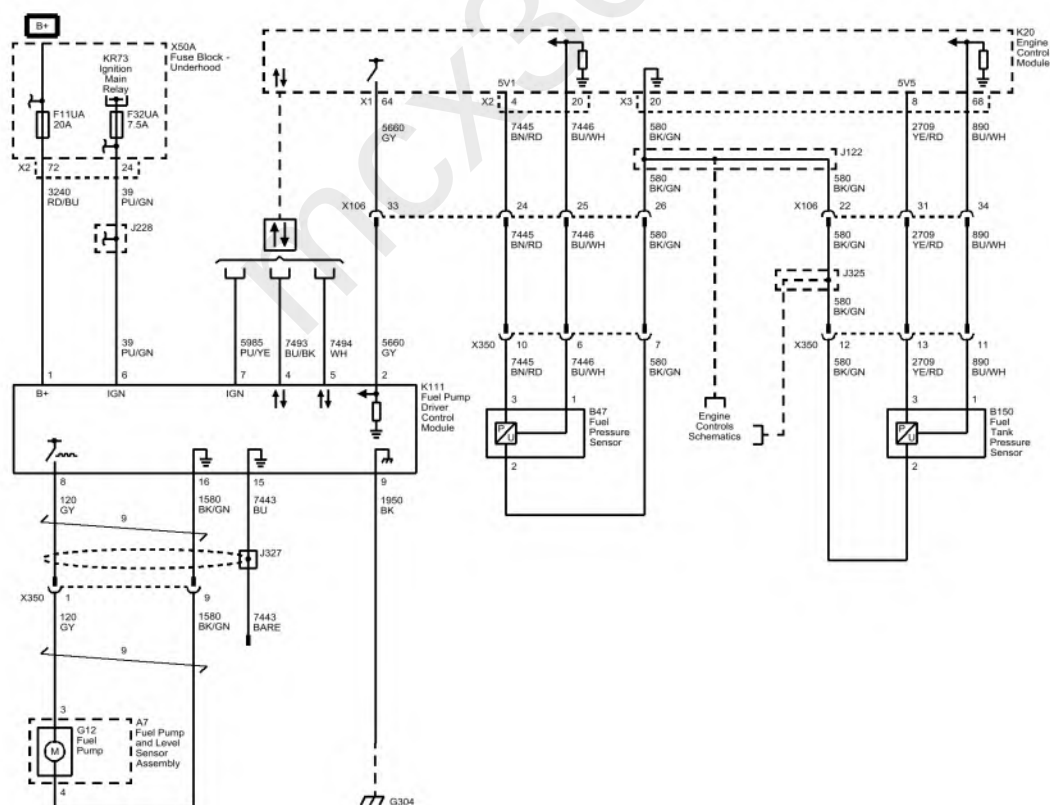
Fig. 11: Fuel Controls - Fuel Pump and Fuel Pump Controls Courtesy of GENERAL MOTORS COMPANY
